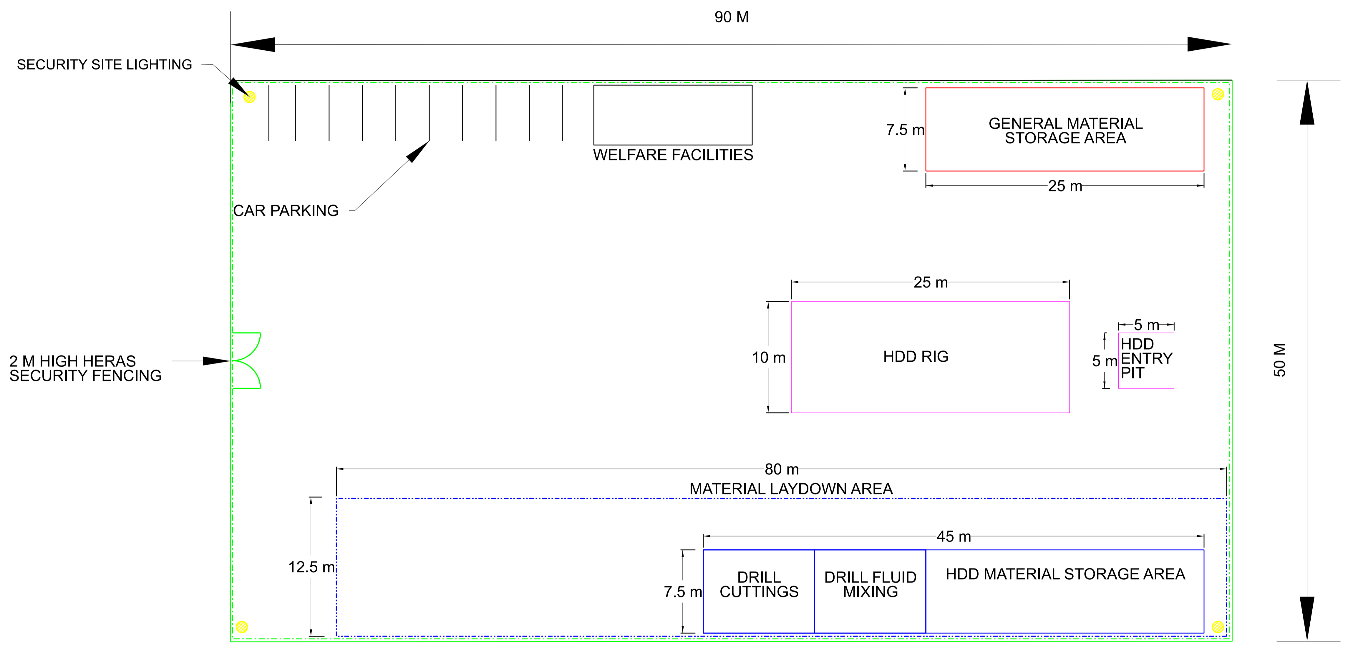
TEMPORARY HORIZONTAL DIRECTIONAL COMPOUND/ LAYDOWN AREA SCALE 1:200
